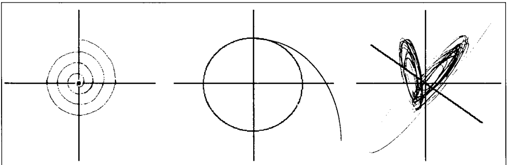
Fig. 2. An attractor can be regarded as the long-term behaviour of a dynamic system in state space, but also as a determinant of the system, that attracts the trajectories of different initial conditions and controls their future development. The two simplest kinds of attractors are the fixed point (left) and the closed curve, or limit cycle (middle). Strange attractors (i.e. chaotic attractors) have a much more complicated structure and correspond to unpredictable motion (right). (Ill. by Gerding after Ruelle 1994)
