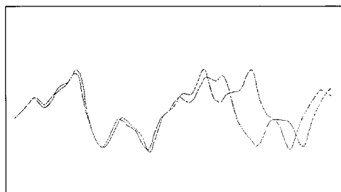
Fig. 1. Chaos was not made apparent until computers first arrived and computer simulations of non-linear systems could be made. When the meteorologist Edward Lorenz wanted to make a rerun of a weather simulation on his computer in 1961, he expected exactly the same result as in the first run. To save time, he typed in the initial value manually, using the numbers from an earlier print-out. As he came back to look at the result he was shocked to find a completely different weather sequence. Lorenz had used a figure with three decimals whereas the computer memory worked with six decimals, causing an infinitely small, but crucial change in the initial value. (Ill. by Gerding after Lorenz 1963)
