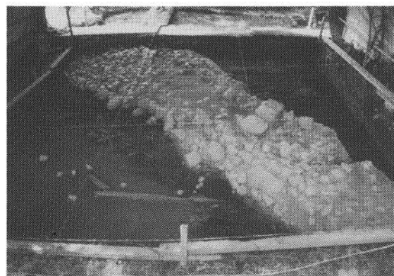
Photo 2. A 2 m wide stone foundation laying on a wooden supporting structure.
