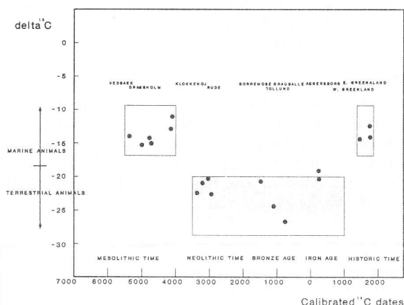
Fig 2. Human delta ^{13}\text{C} values from people in Denmark and Greenland versus calibrated ^{14}\text{C} dates of the samples from Tauber (1981:a)
