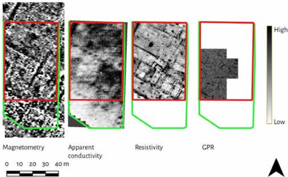
Fig. 7. Comparison of survey techniques at Area A. Red rectangle marks the extent of the resistivity survey, green polygon the extent of the conductivity survey. Plots by D. Pitman and R. Potter.
