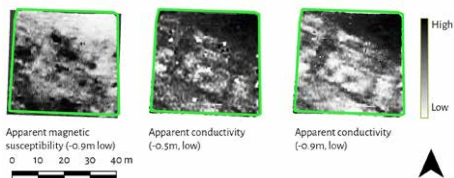
Fig. 4. Results of EM survey, Area B. Plots by D. Pitman.
