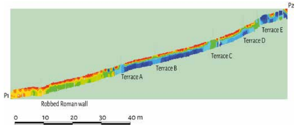
Fig. 6. EM profile (pseudo-section) showing the location of possible terraces and the line of the robbed-out Late Roman wall. The locations of P1 (south) and P2 (north) are shown on Fig. 2. Section by D. Pitman.
