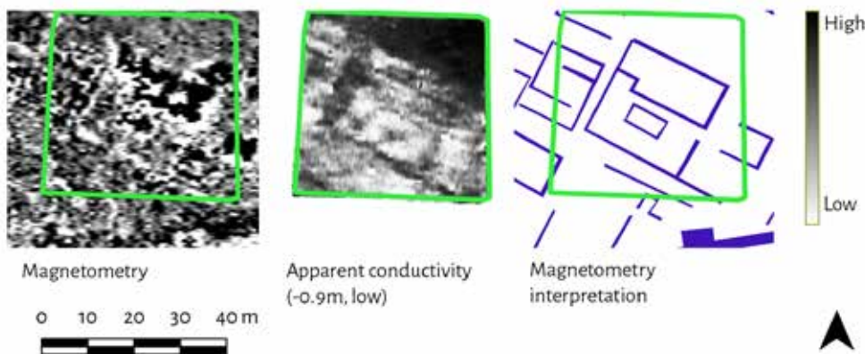
Fig. 8. Comparison of survey techniques at Area B, with interpretation of magnetometric results. Area marked with green corresponds to extent of conductivity survey. Plots by D. Pitman and R. Rönnlund.
