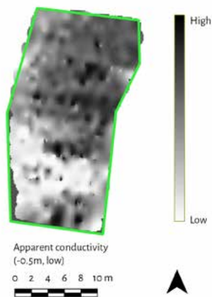
Fig. 5. Results of EM survey of Area C. Plot by D. Pitman.
