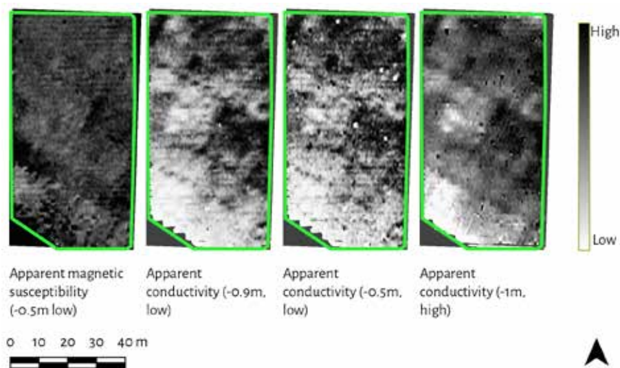
Fig. 3. Results of EM survey, Area A. Plots by D. Pitman.
