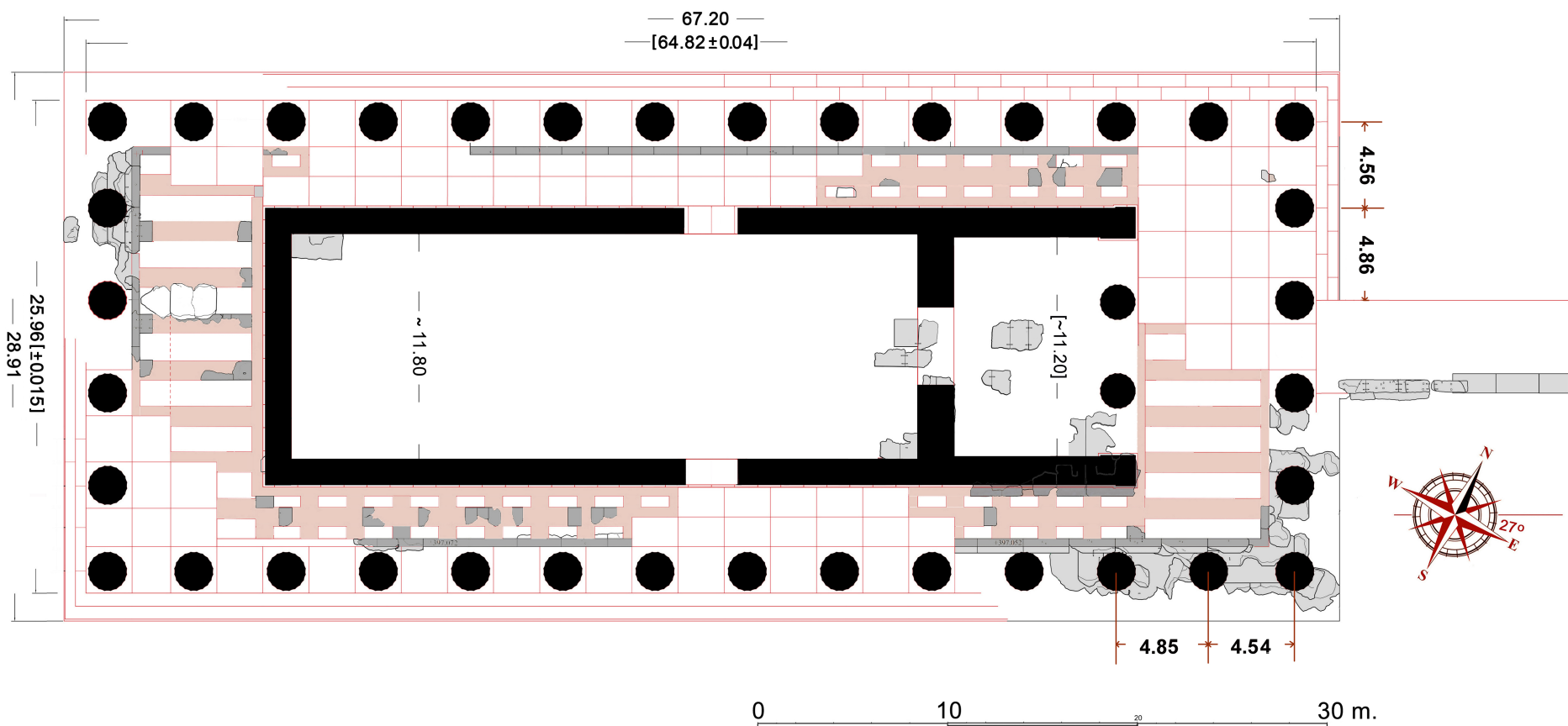
Fig. 10. Reconstructed ground plan of the Temple of Zeus. The location of the lateral doorways is hypothetical. In grey, the extant remains; in pink, the reconstructed layout of the grid blocks. Illustration by C. Kanellopoulos.
