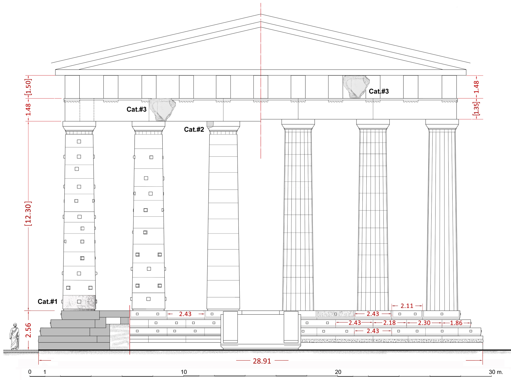
Fig 11. Reconstructed elevation of the Temple of Zeus incorporating the extant drum, and fragments of the capital and entablature. Reconstructed dimensions in brackets. Illustration by C. Kanellopoulos.
