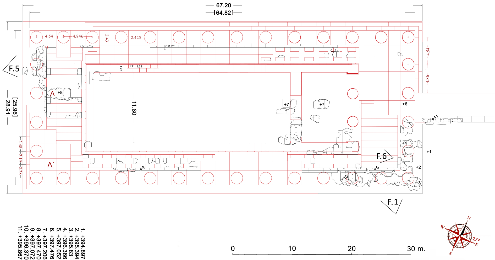
Fig. 9. The ground plan of the Temple of Zeus; in black the extant remains; in red the reconstructed features. F.1, F.5 and F.6 are the viewpoints of Figs. 1, 5, 6. Illustration by C. Kanellopoulos with L. Tsatsaroni and N. Georgakopoulou.
