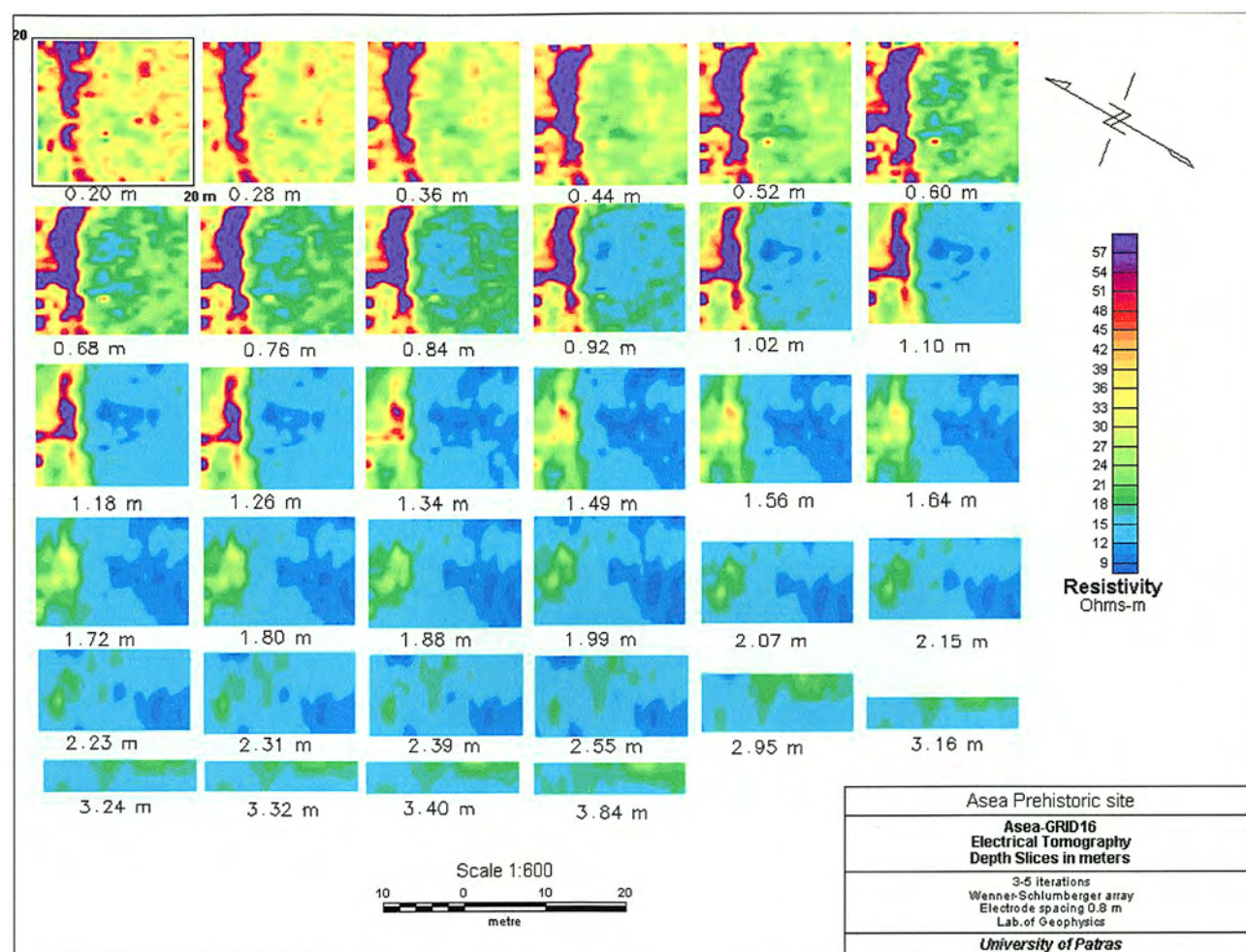
Fig. 5. City-gate complex in the SW, eastern part, using electrical tomography, showing depth slices in meters in square 16.
