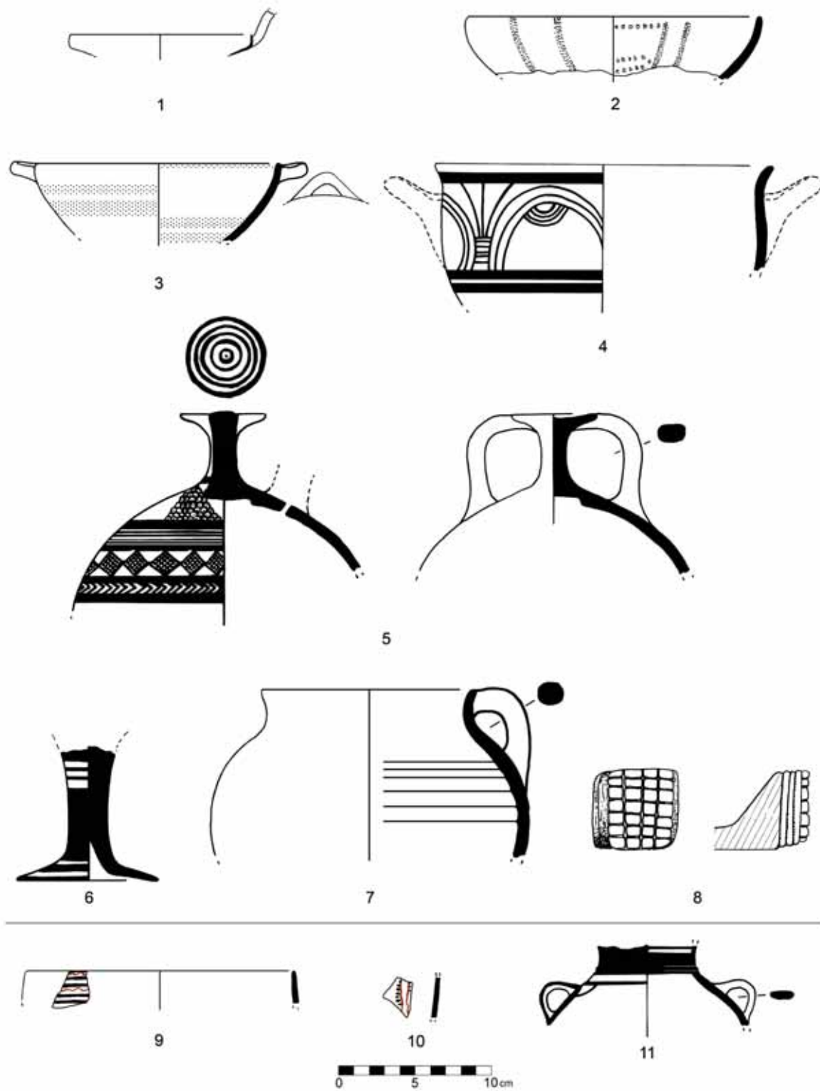
Fig. 7a. Collection of finds from Stratum 1, Area 6 West. Finds below line (9–11) are residual (drawing by M. Al-Bataineh).
